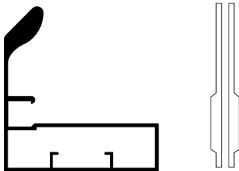
Product Code: DV.SHAP.81 45mm Left/Right Handle Profile (CNC) Size: 3100 mm
