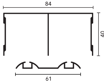
TOP & BOTTOM TRACK Top Track: DV.WRAP.104/105 Bottom Track: DV.WRAP.106/107 Length: 3000 mm / 4000 mm
