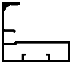
Product Code: DV.SHAP.80 45mm Center Handle (CNC) Size: 3100 mm
