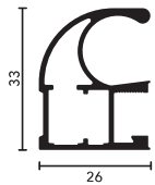
C TYPE HANDLE DV.WRAP.100 Length: 3000 mm
