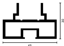
Horizontal Profile DV.SPAP.101 Available Finish: Ceramic Black/Brush Gold Matt
