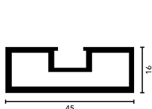
Vertical Profile DV.SPAP.100 Available Finish: Ceramic Black/Brush Gold Matt
