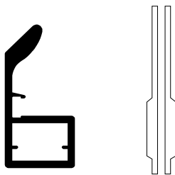
Product Code: DV.SHAP.78L/78R Slim Left/Right Handle Profile (CNC) Size: 3100 mm
