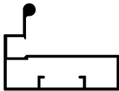
Product Code: DV.SHAP.65 45mm Frame Handle Profile (Bindi) Size: 3000 mm
